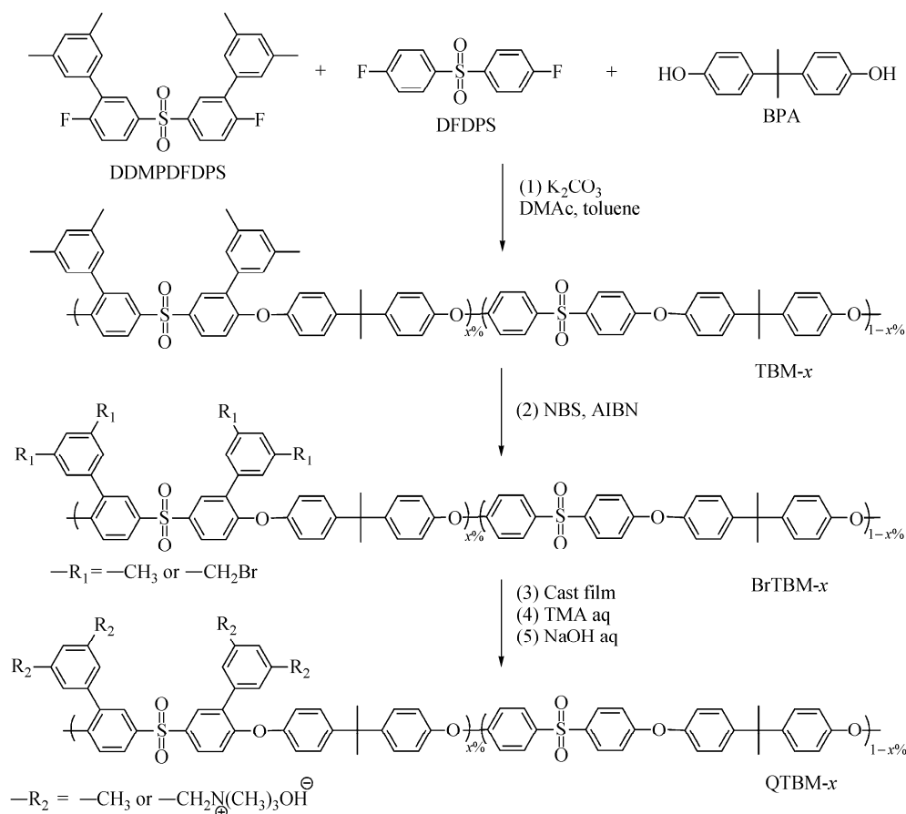
Scheme 2 Synthetic route to poly(arylene ether sulfone)s ionomers QTBM s
