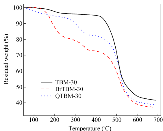
Fig. 7 TGA curves of TBM-30, BrTBM-30 and QTBM-30
